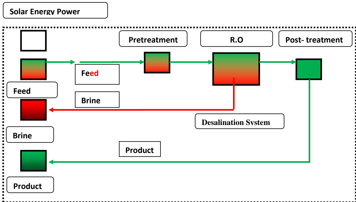
Figure 10: Typical schematic diagram of R.O Desalination System(ADAN, 2011).
