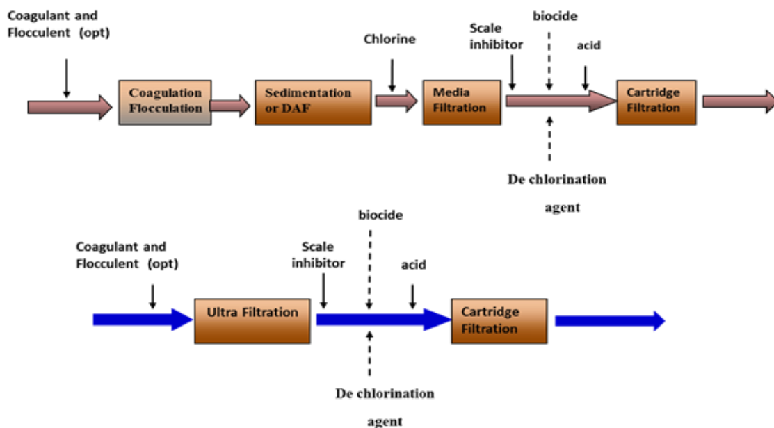
Figure 11: Typical pretreatment possible schemes, Source: (ADAN, 2011).
