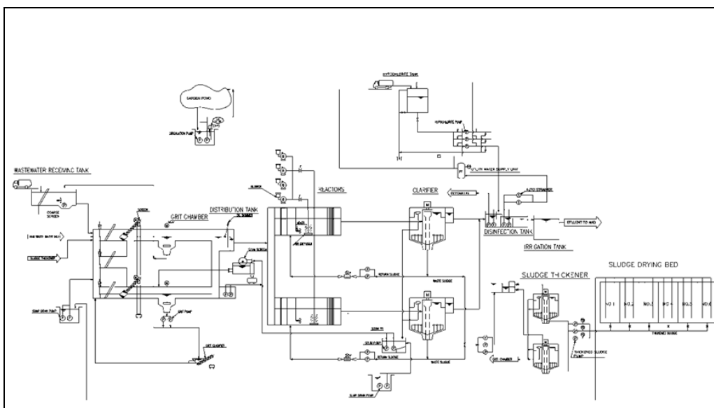
Figure 26 : JWWTP- Treatment Flow Sheet, Source: (NJS, 2013).
