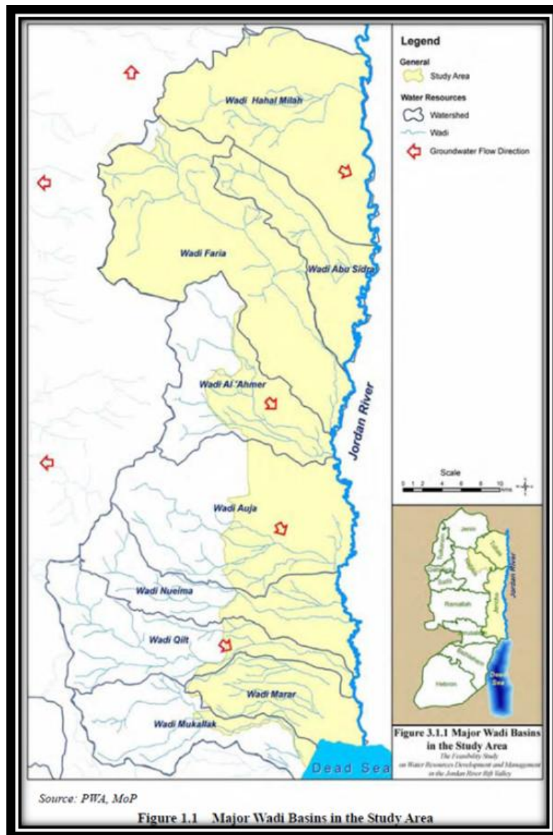
Figure 32: Major wadi basins in the study Area (PWA, 2013).
